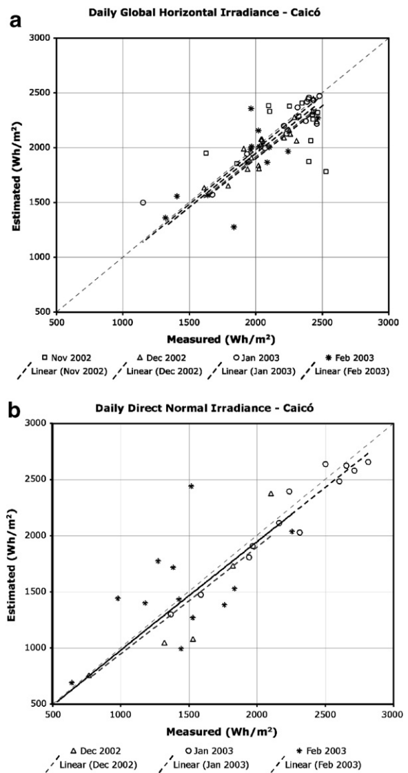
Fig. 2. (a) Comparison among estimated and measured global irradiance at Caicó/PE. (b) Comparison among estimated and measured direct normal solar irradiance for the same location.
