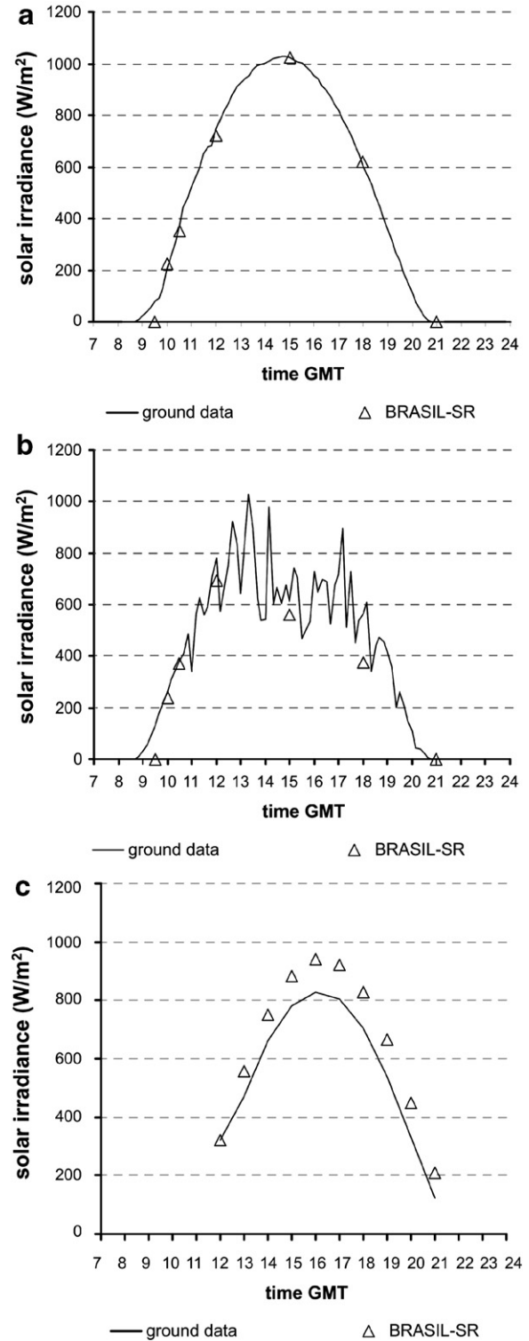
Fig. 4. Plots of daily cycle of global solar irradiation for (a) clear sky day in Petrolina; (b) overcast day in Petrolina and (c) clear sky day in Cuiabá. Continuous line represents the ground data and triangles are the estimated values provided by BRASIL-SR model at the GOES-12 image times.
