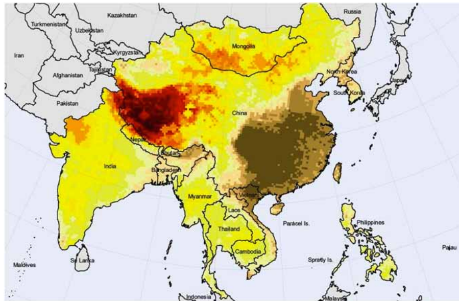
Figure 59 Solar and Wind Energy Resource Assessment in China – SWERA Project
