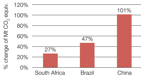
Figure 2 Percentage Change in GHG Emissions From 1990 To 2007
