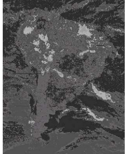
Figure 1: Image from the visible channel of the GOES-EAST satellite
