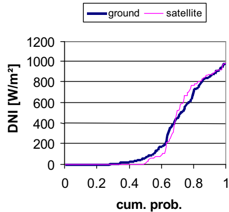
Figure 4 Comparison of the cumulative distributions of the ground (thick line) and satellite derived data of the hourly direct normal irradiance. This example refers to the site Caicó, month of January. The satellite derived data are gained with the SUNY model from GOES images.
