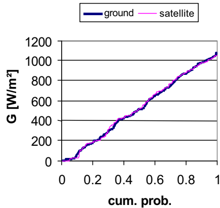
Figure 3 Comparison of the cumulative distributions of the ground (thick line) and satellite derived data of the hourly global irradiance data. This example refers to the site Caicó, month of January. The satellite derived data are gained with Heliosat from METEOSAT images.
